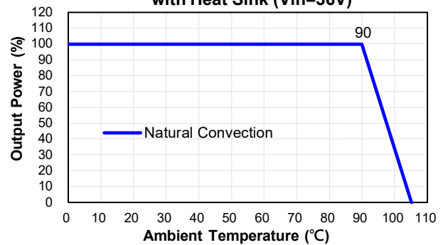
CQB50W8-36SXX-CMFD+HS(HD) Derating Curve with Heat Sink (Vin=36V)
