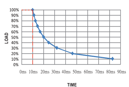
RSD-100C-24
