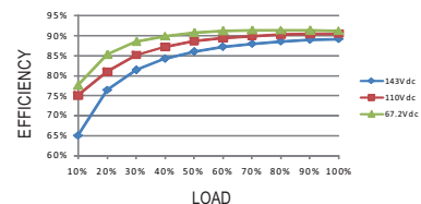
RSD-100D-24
