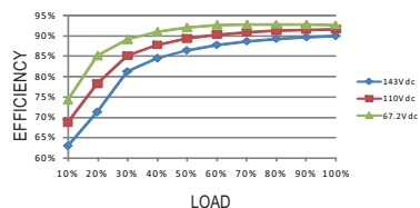
RSD-100D-12
