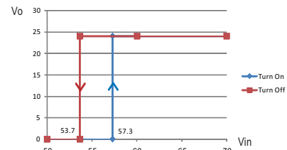
RSD-100D-24
