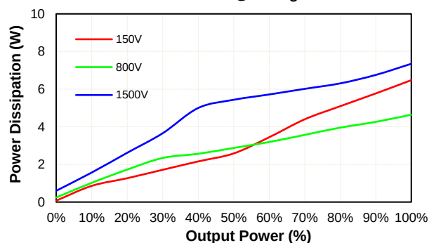
DH45W10-800S24 Pd Vs Po @25 Deg. C
