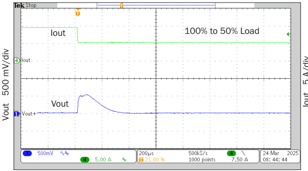
200 \mu s/div cMOR2812S step load response FIGURE 49
