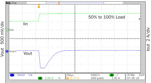
100 µs/div cMOR2828S step load response
