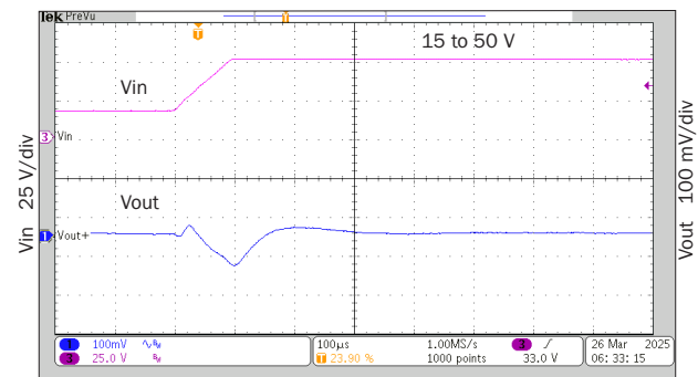
100 μs/div cMOR2805S step line response
