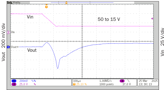
100 µs/div cMOR2828S step line response
