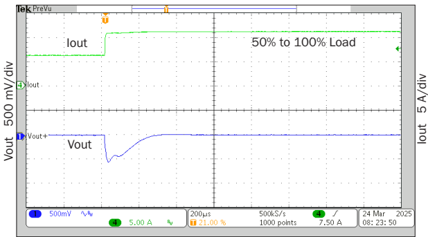
200 \mu s/div cMOR2812S step load response FIGURE 48
