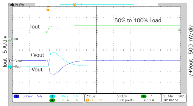
200 \mu s/div cMOR289R5D step load response FIGURE 72
