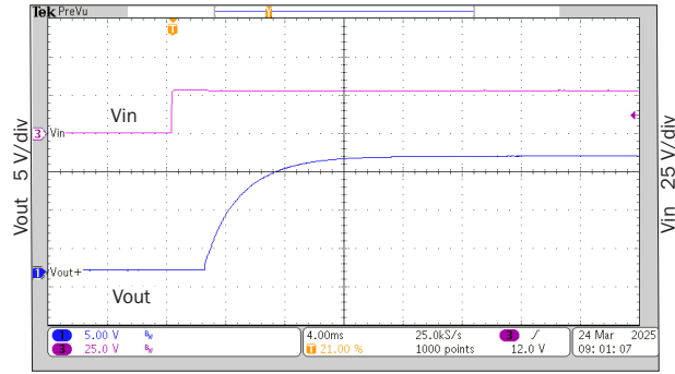
4.00 ms/div cMOR2815S start-up response FIGURE 51
