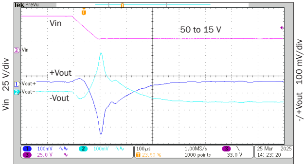
100 \mu s/div cMOR2815D step line response FIGURE 83
