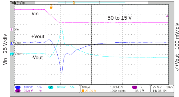
100 \mu s/div cMOR2812D step line response
