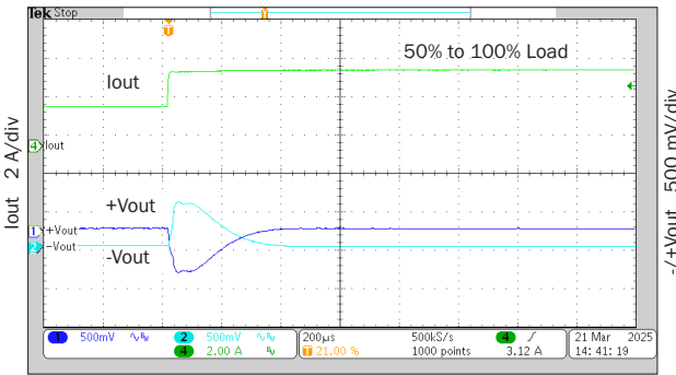
200 \mu s/div cMOR2815D step load response FIGURE 84
