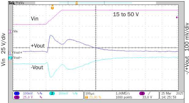
100 \mu s/div cMOR2815D step line response FIGURE 82
