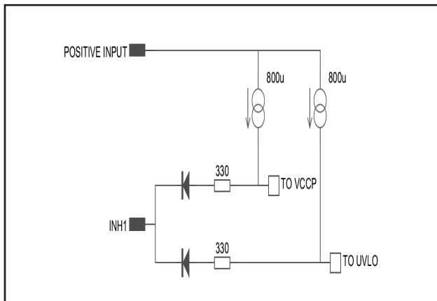
FIGURE 4: INH1
