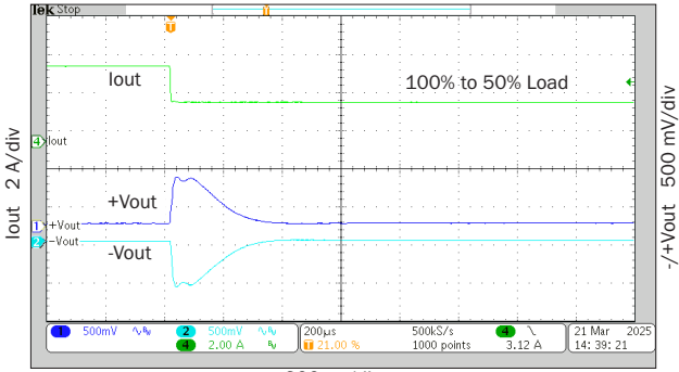
200 \mu s/div cMOR2815D step load response FIGURE 85
