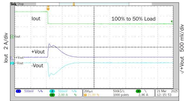
200 \mu s/div cMOR2812D step load response
