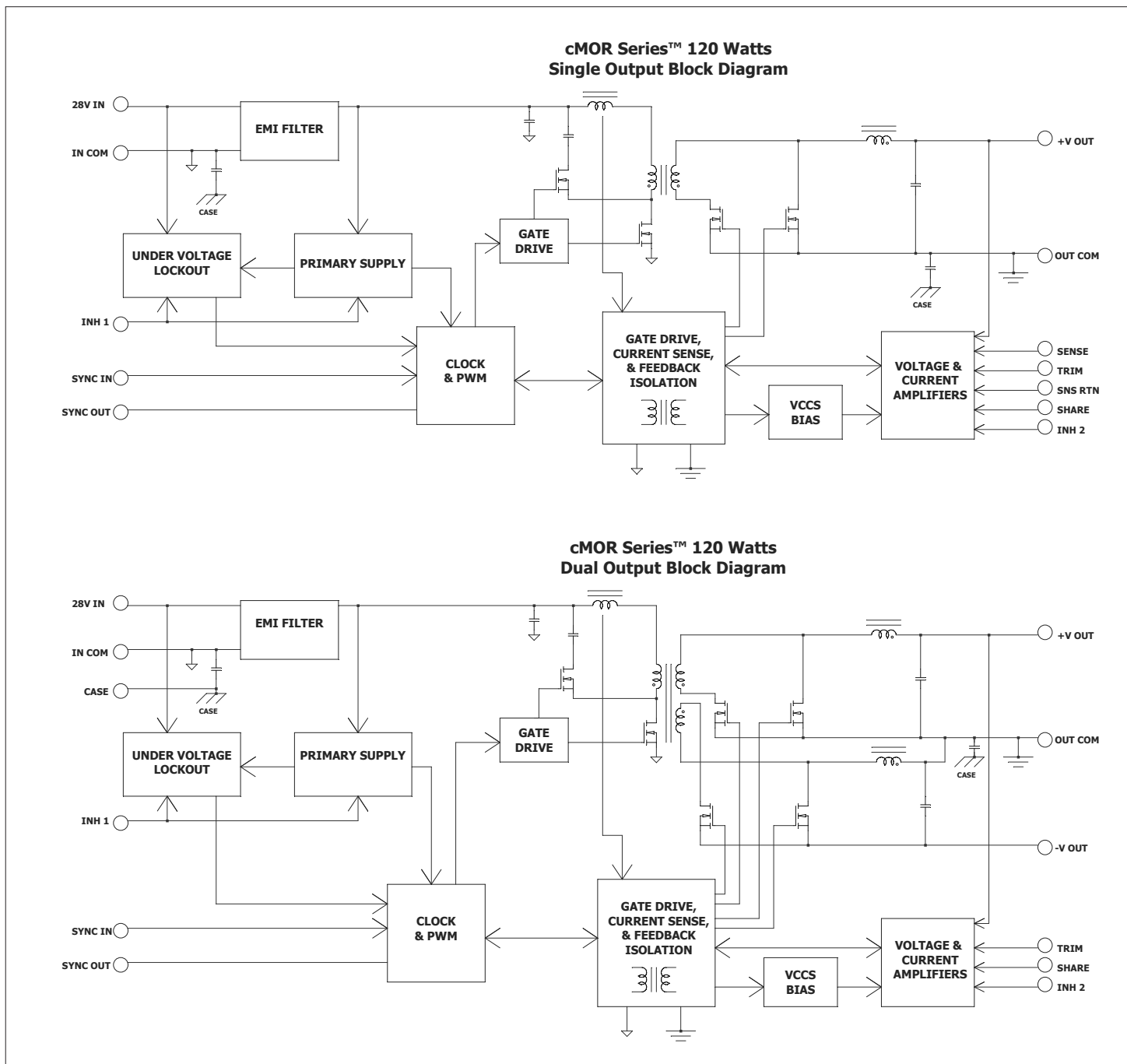
Figure 13: cMOR Single And Dual Output Block Diagram
