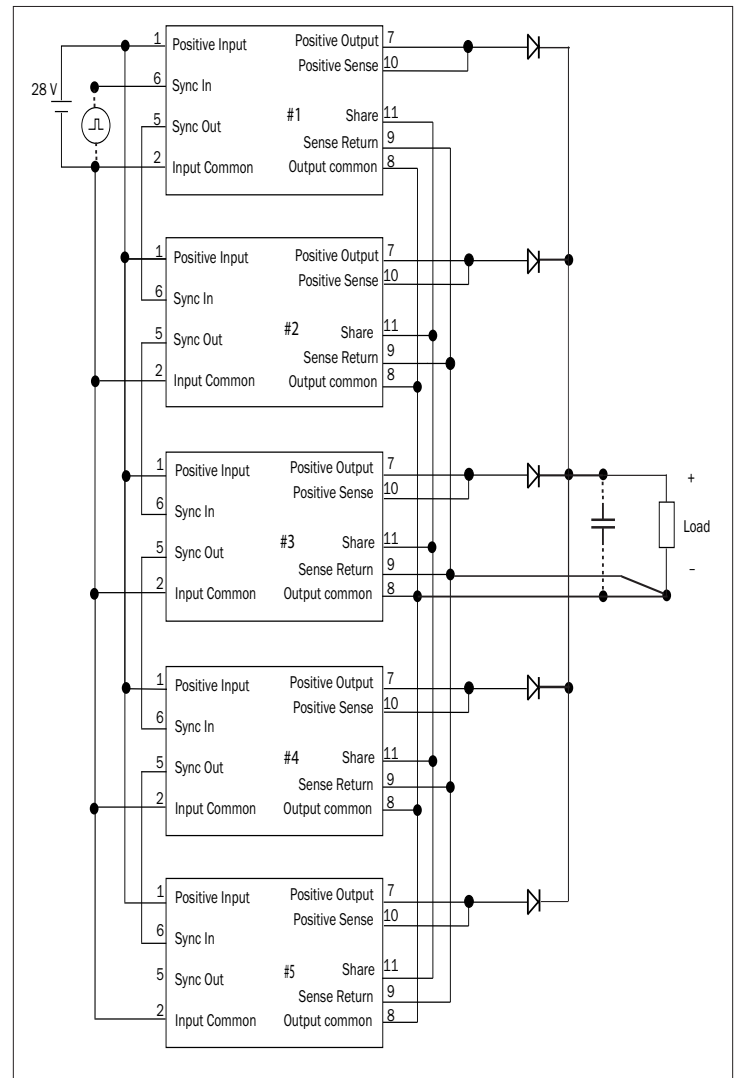
FIGURE 8: PARALLELING
