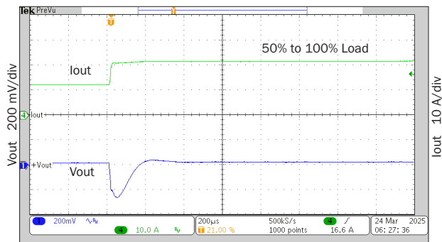
100 μs/div cMOR2805S step load response
