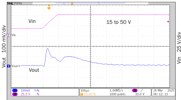
100 \mu s/div cMOR2812S step line response FIGURE 46
