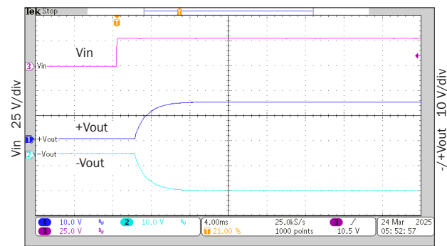
2.00 ms/div cMOR2815D start-up response
