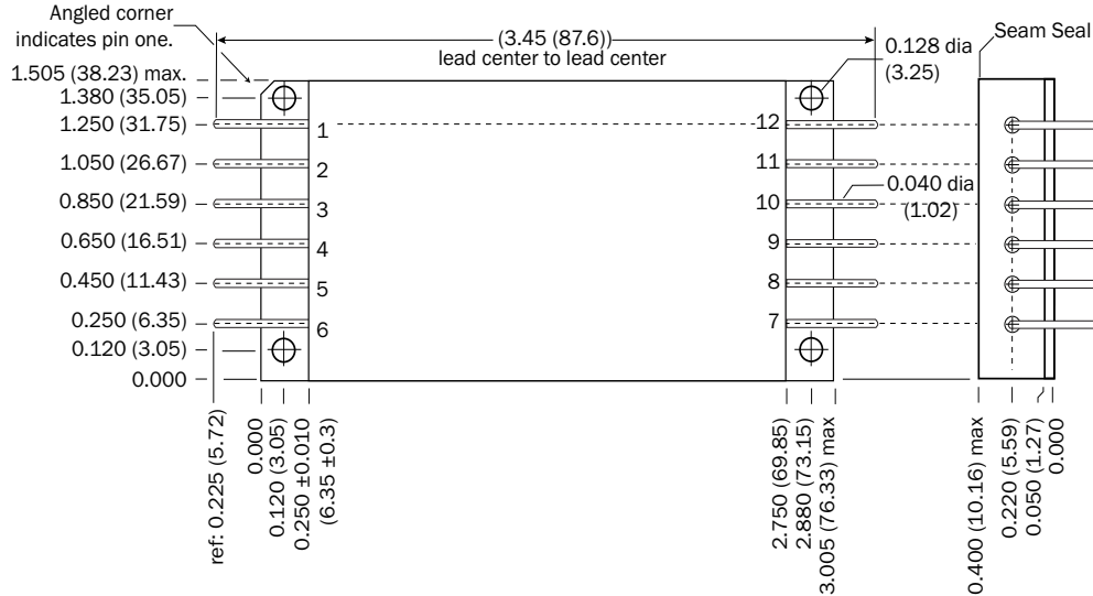
TOP VIEW CASE V Flanged case, down leaded
