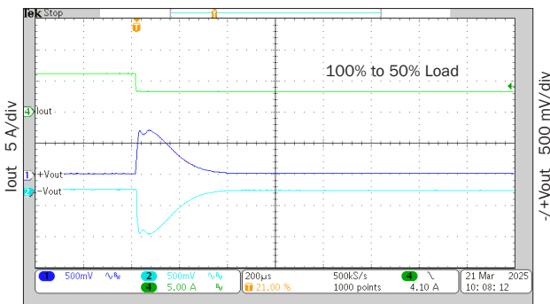
200 \mu s/div cMOR289R5D step load response FIGURE 73
