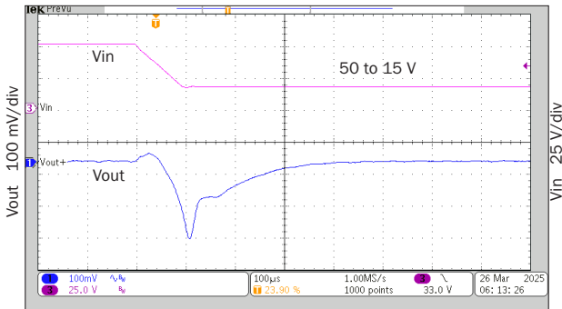
100 \mu s/div cMOR2812S step line response FIGURE 47
