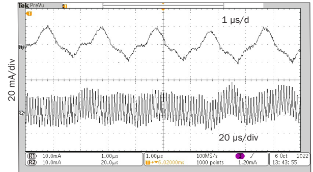
1 μs/div cMOR2805S Input Ripple Current (Iin)
