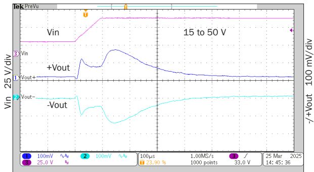
100 \mu s/div cMOR289R5D step line response FIGURE 70
