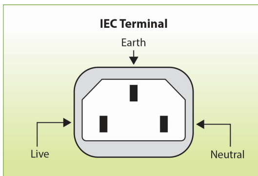
Option 1 (IEC Terminal)
