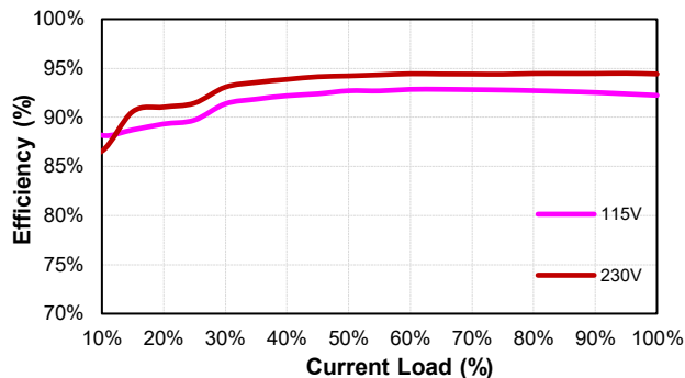
LFM420S360 (Eff Vs Io)
