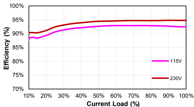
LFM420S540 (Eff Vs Io)
