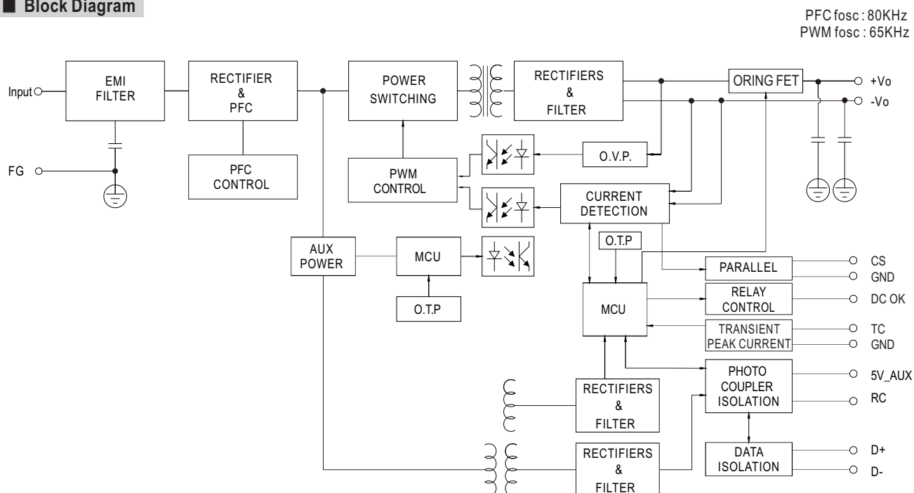
Suitable for 220/230/240/277Vac System (180~305Vac)
