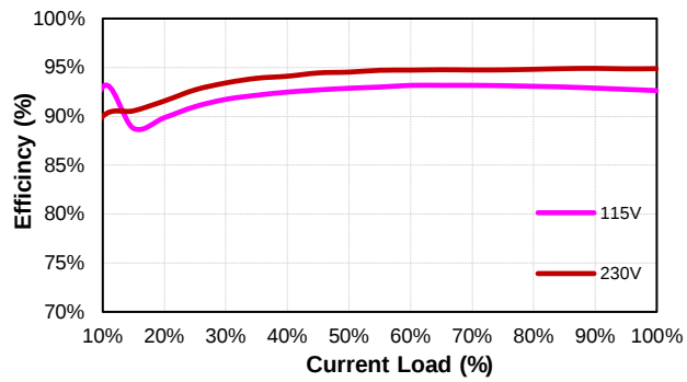
LFM420M480 (Eff Vs Io)
