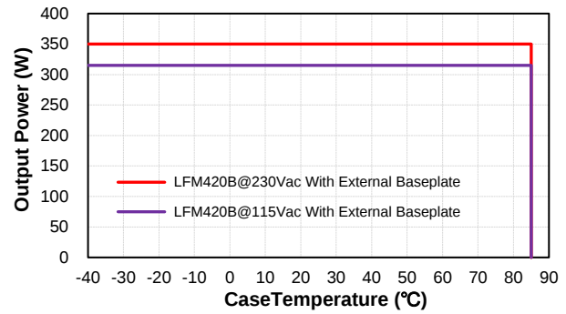
Output Power vs CaseTemperature
