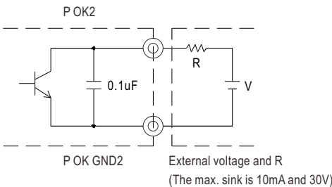
Fig. 4.2 Internal circuit of P OK2 (Open collector method)
