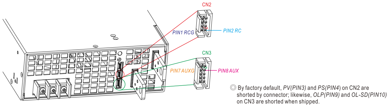
Example 3.2(A): Using external voltage source
