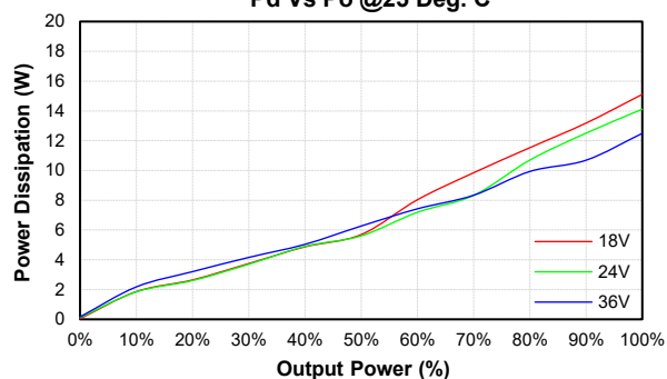
CHM150-24S12 Pd Vs Po @25 Deg. C
