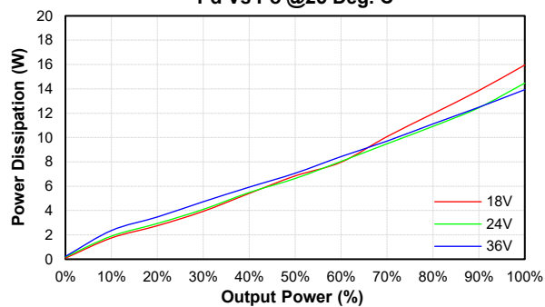
CHM150-24S24 Pd Vs Po @25 Deg. C
