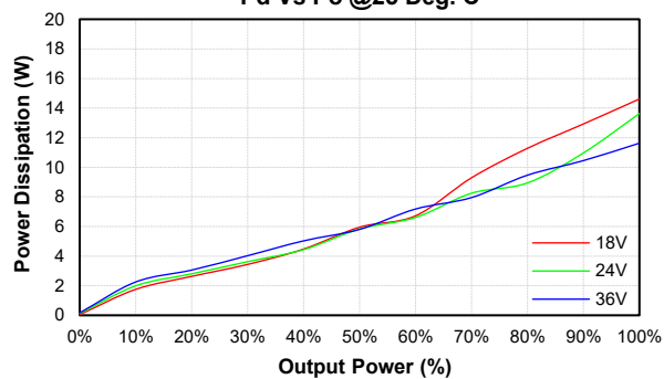
CHM150-24S15 Pd Vs Po @25 Deg. C
